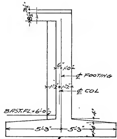
SECTION FF.
